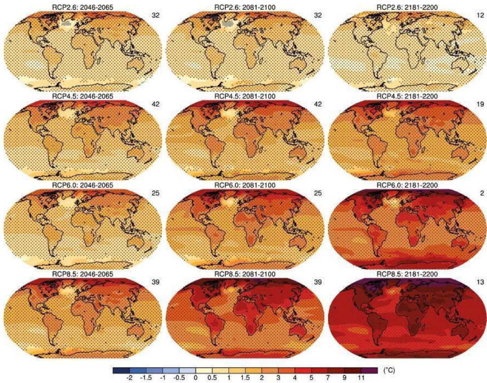
Figure 3-2: Predicted temperature changes under various RCP scenarios.
